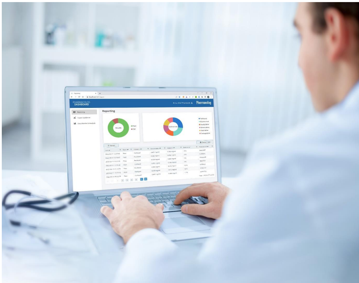
Figur 6 - Pharmacolog Dashboard™
